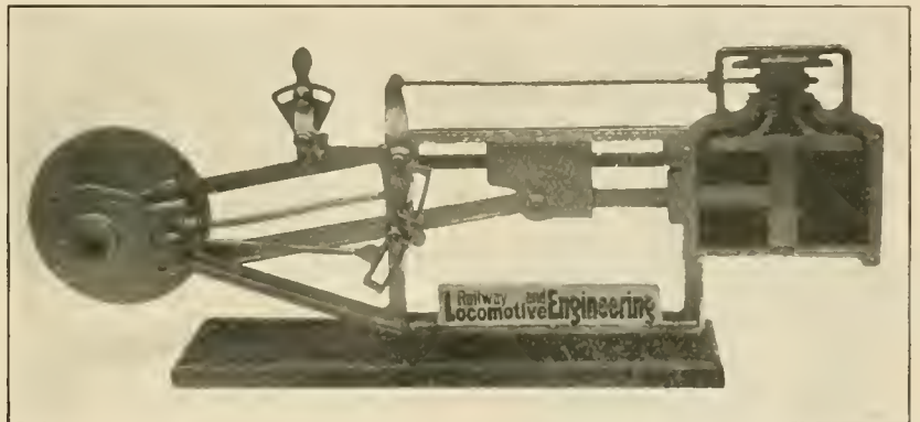
ANGUS SINCLAIR COMPANY'S VALVE MOTION MODEL.
